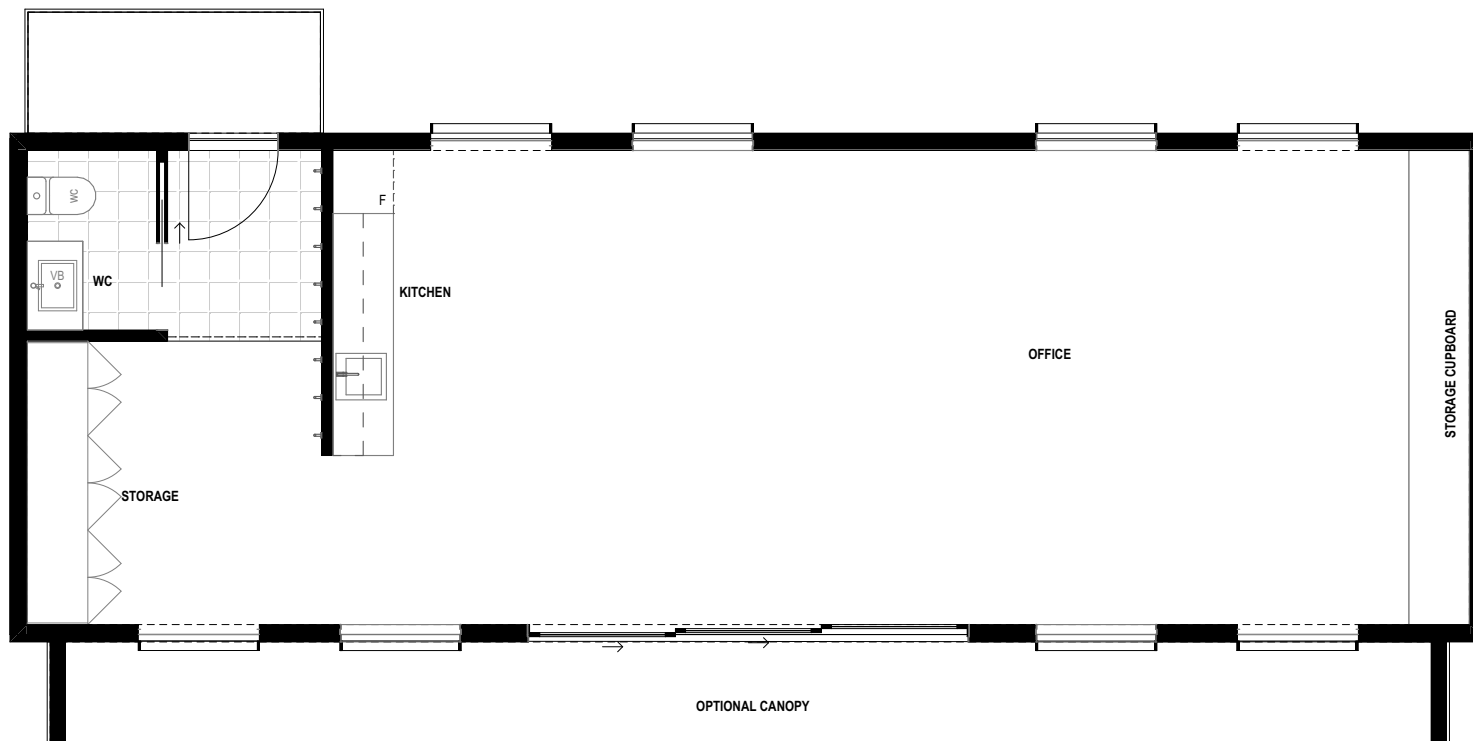
FLOOR PLAN
