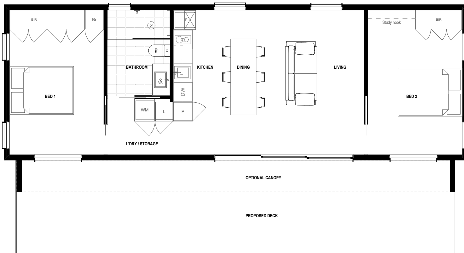
FLOOR PLAN
