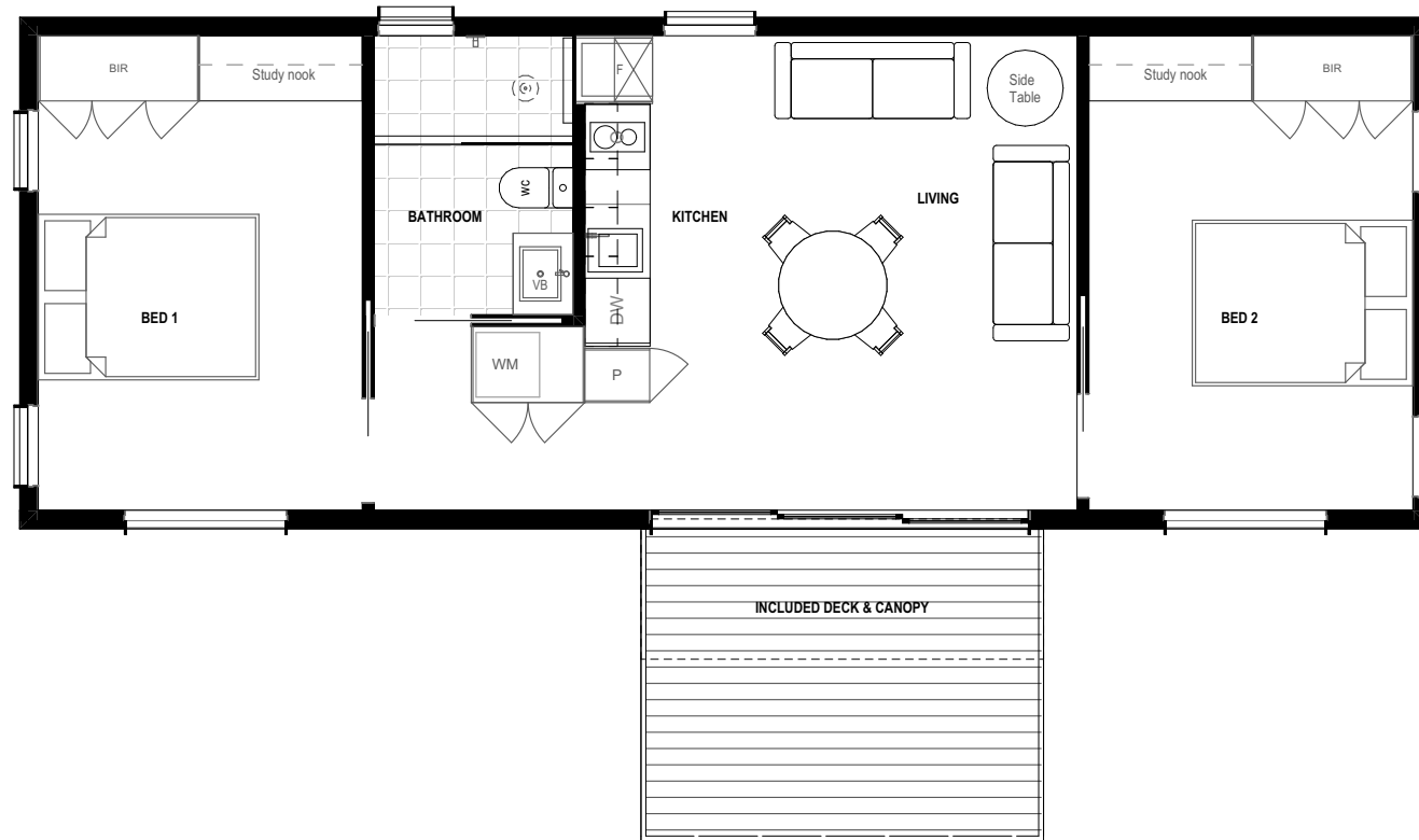
FLOOR PLAN
